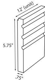
Top rail 6" Base rail 6"
