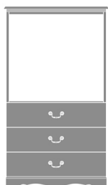
Charlotte Armoire, 3 Drawers, No Doors Model: CHAM30 35.5W 23.75D 63.5H
