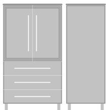
Chicago Armoire, 3 Drawers, 2 Doors Model: CCAM32 35.5W 23.75D 63.5H
