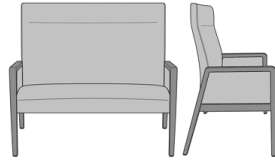
Valdina Bariatric Chair, Tall Back, with Upholstered Arm Panels - 46" W Moasdfadel: VLDFIXB46PUP 46W 27.5D 35H 26AH
