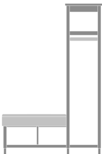
Ethan Wardrobe with Bench, No Drawers, No Doors, Metal Leg, Right Sided Moasdfadel: ETNWB00MLR 48W 24.25D 72H
