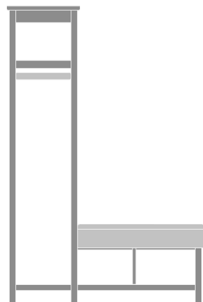
Ethan Wardrobe with Bench, No Drawers, No Doors, Classic Leg, Left Sided Moasdfadel: ETNWB00CLL 48W 24.25D 72H
