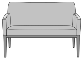
Terrasini Love Seat, with Solid Surface Arm Caps, without Piping, with Concealed Cleanout Moasdfadel: TER241 47W 26.5D 34H 24.75AH
